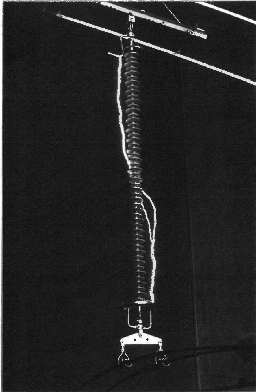
Pict.2: 50% Lightning impulse flashover test
