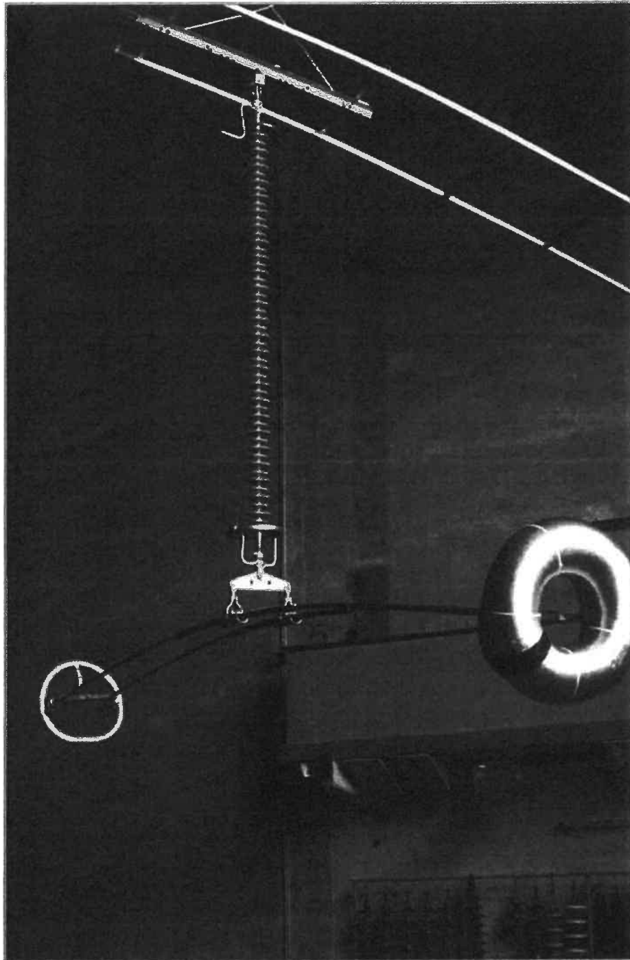
Photo of the test setup
