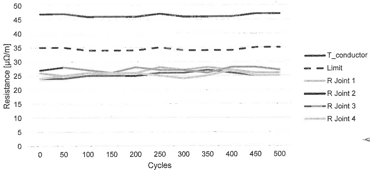
Electr. Resistance of Compression Joints
