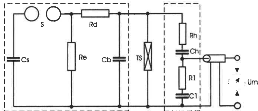
Circuit diagram for test with lightning impulse voltage 1,2/50 μs and switching impulse voltage 250/2500 μs
